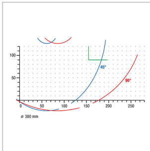
Double mitre saw DG 79 Cutting diagram DG 79
